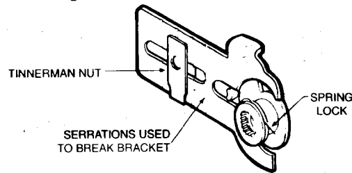
Figure 2 Tinnerman Nut Spacing and Serration Breakoff
